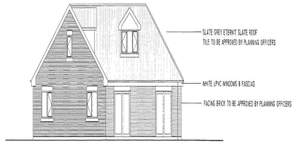
WEST ELEVATION
