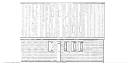
NORTH ELEVATION
